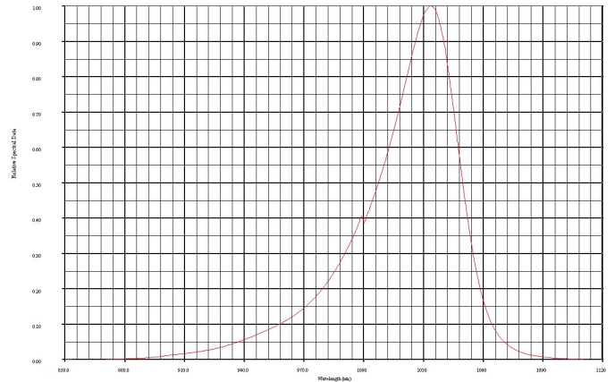
SPECTRAL RESPONSE
